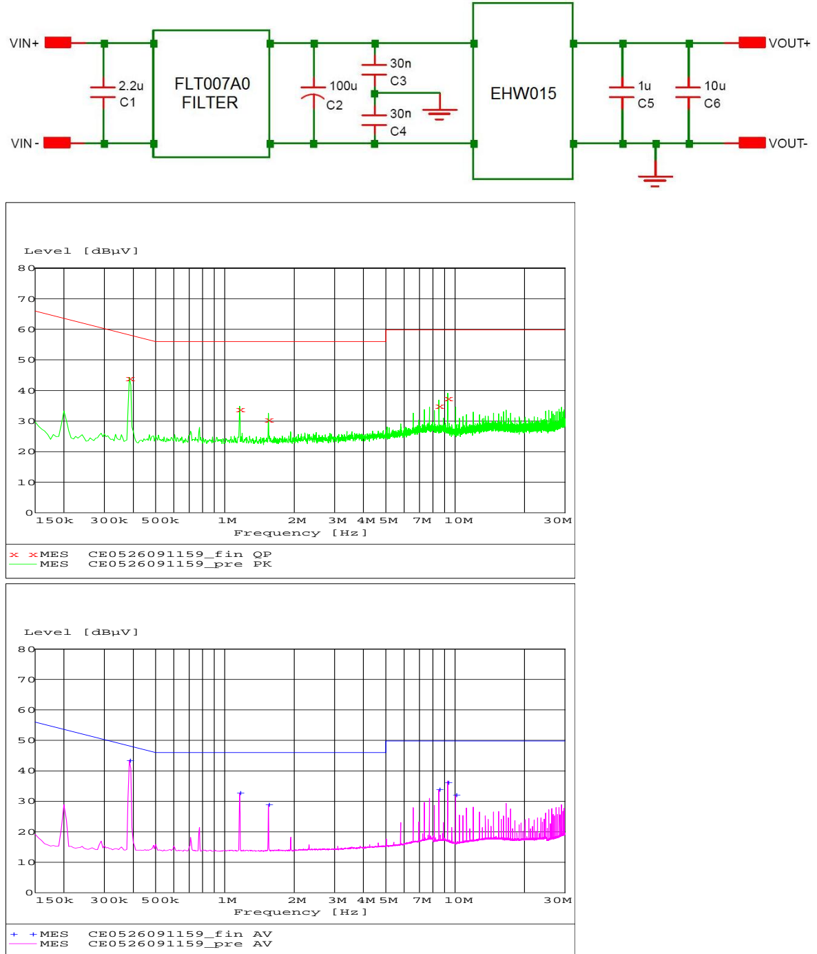
Figure 28. EMC Considerations
